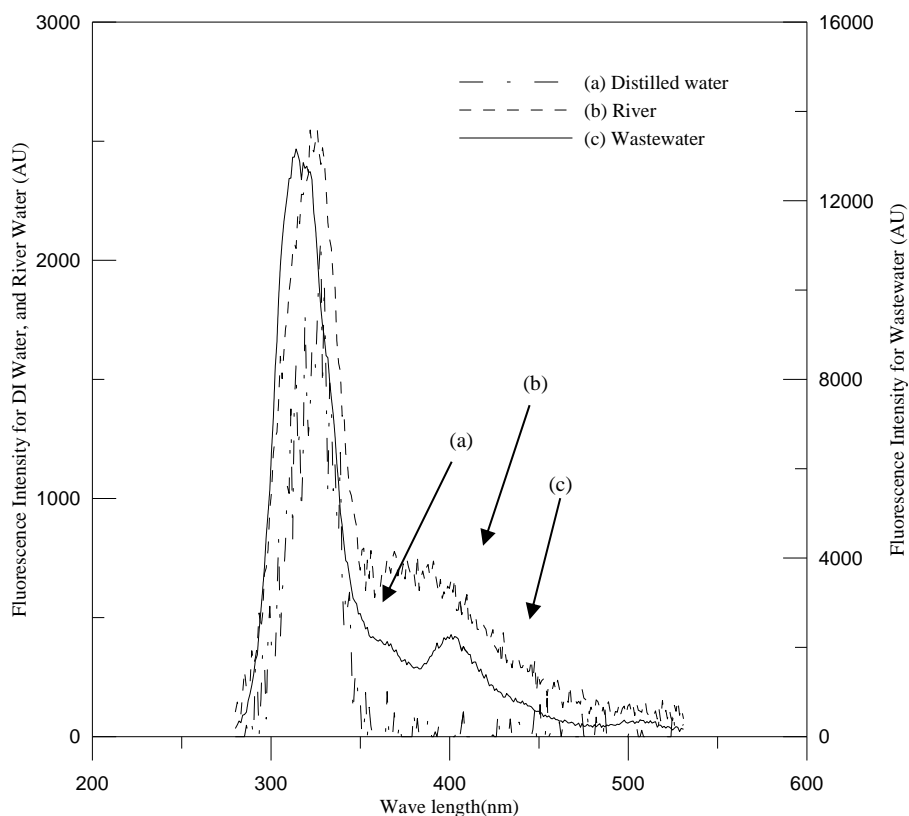
FIGURE1: Synchronous fluorescence spectra of (a) DI water (b) river water, and (c) wastewater
