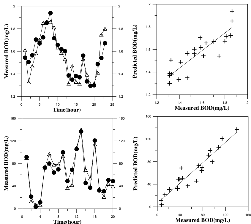
FIGURE 4: Correlation between manually-measured BOD 5 and model predictions for (a) river waters and (b) wastewaters
