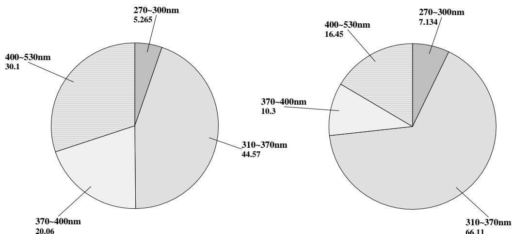
FIGURE 2: Pie-chart of synchronous fluorescence spectra for (a) River water and (b) WWTP effluent
